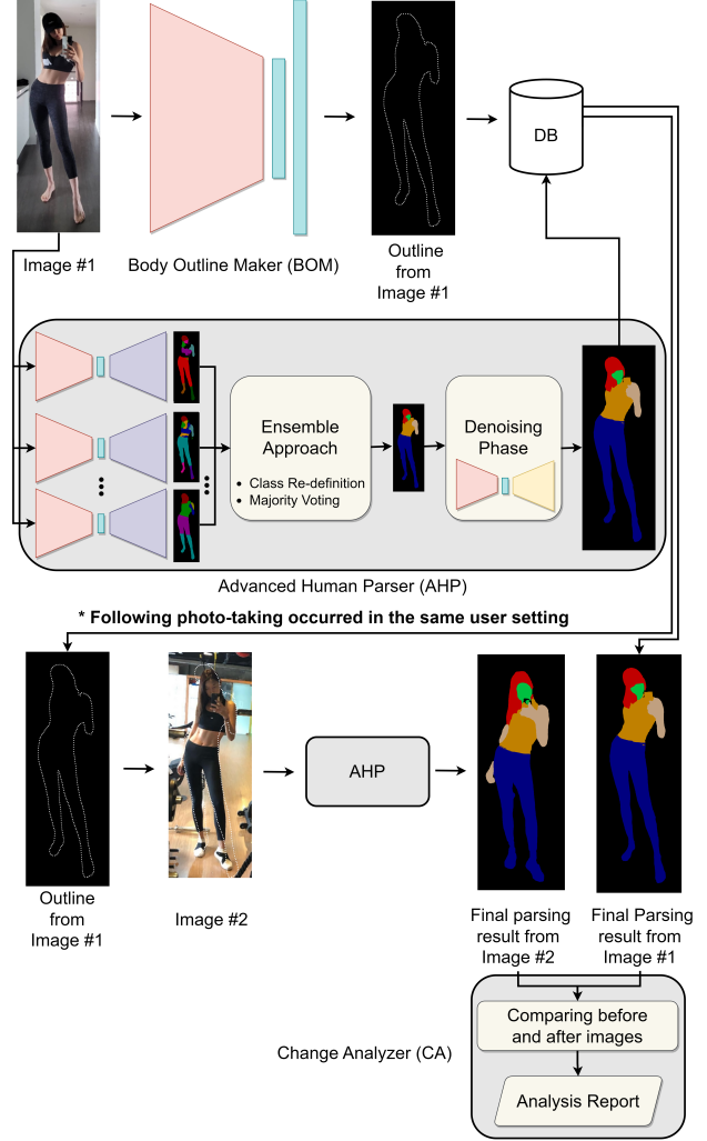
Figure 4. A high-level architecture of AInBody illustrated with examples.
