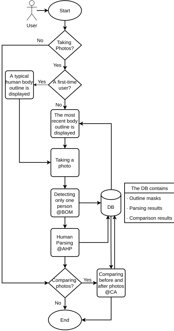
Figure 3. A service flowchart of the proposed AInBody solution.
